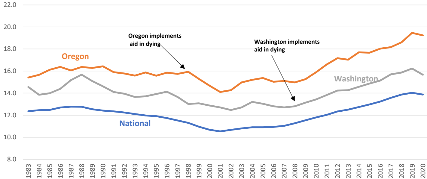
Suicide Rates 1983-2020 -- Oregon, Washington, National Age-Adjusted, 3-Year Moving Average
